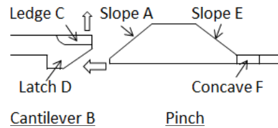
Fig. 8 Insertion of plug.
