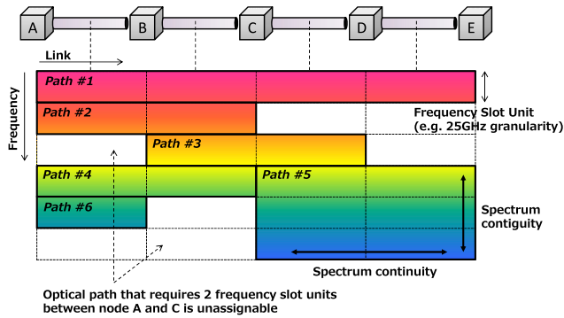
Fig. 3 Spectrum assignment of elastic optical paths.
