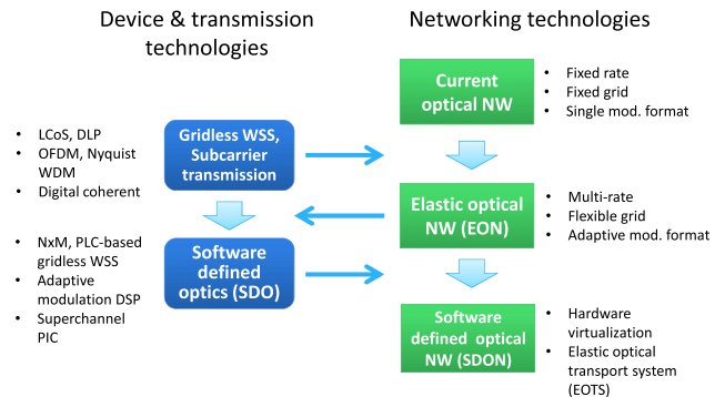
Fig. 1 Optical networking evolution.
