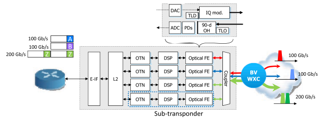
Fig. 6 Multi-flow transponder architecture example.
