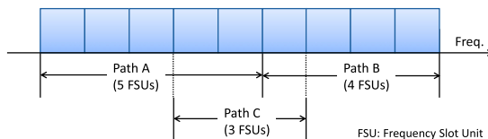
Fig. 5 Partial frequency slot sharing in the shared protection [22].
