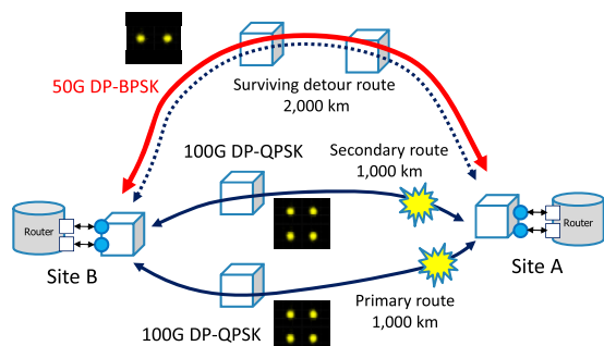
Fig. 4 An example of adaptive modulation.
